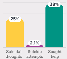
Suicidality 1
